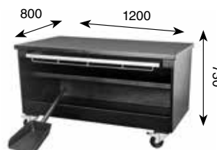
COAL BUNKER TABLE PIRA 120 LUX
